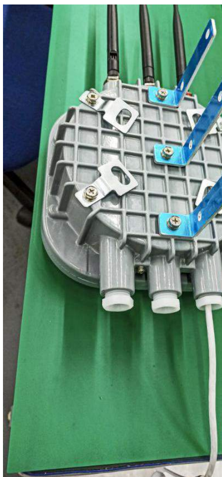
Figure 3.1-L fix L-shape steel on the bottom side
