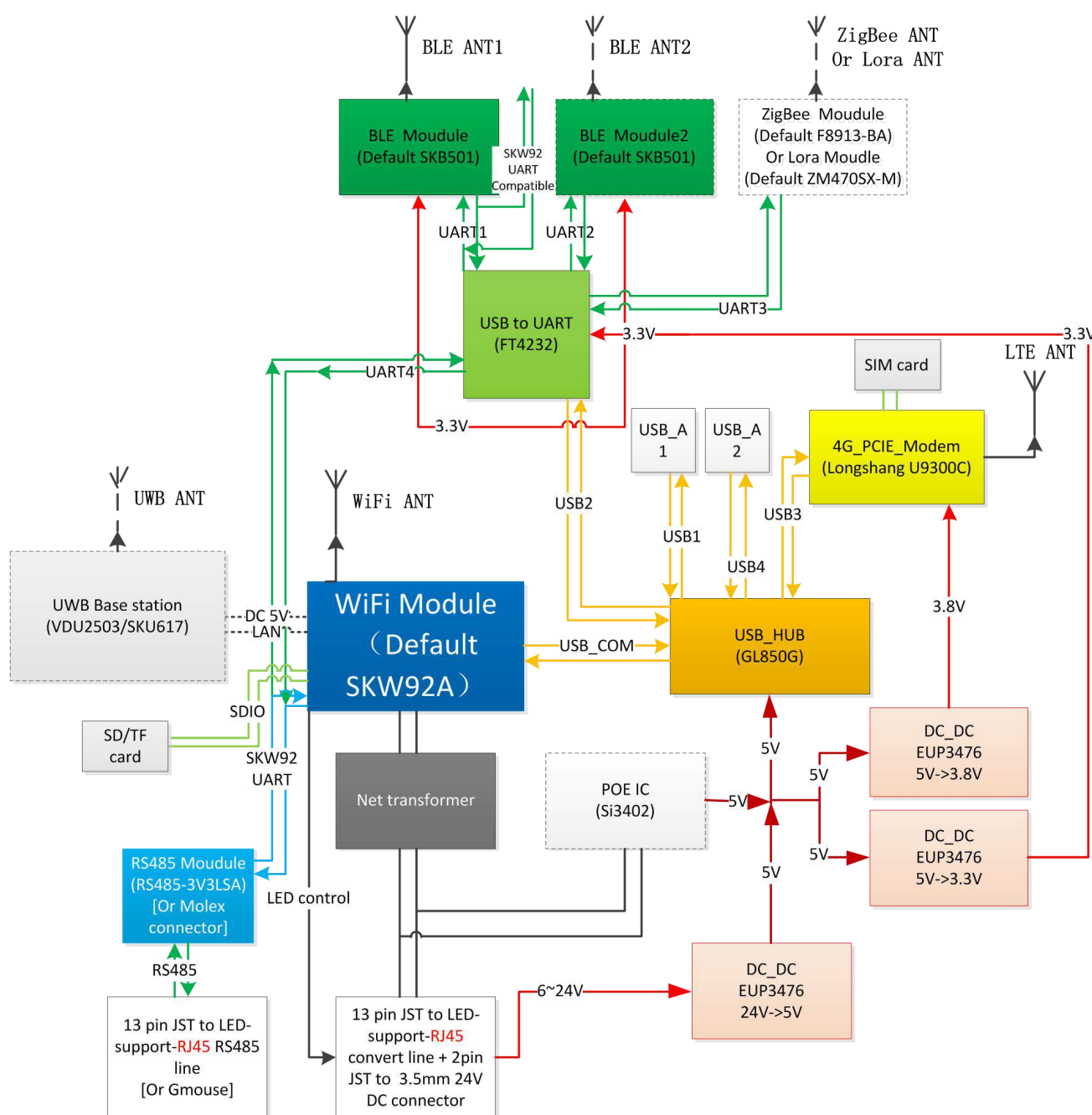
Figure 1.1 系统框架图/Application Diagram
